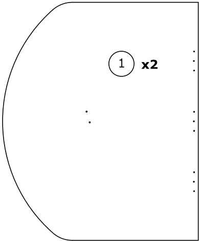
660x800x18mm
