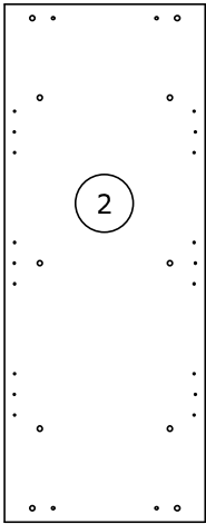
310x800x18mm
